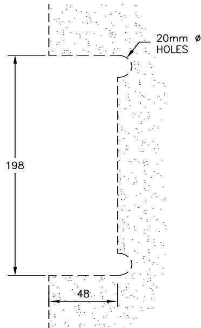
GLASS PREPARATION
