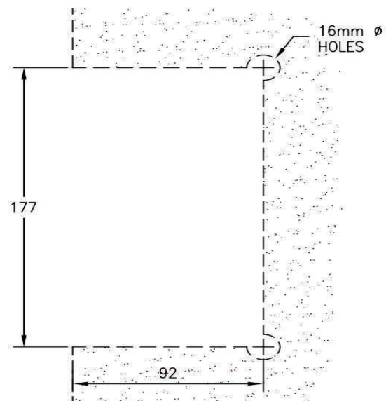
GLASS PREPARATION
