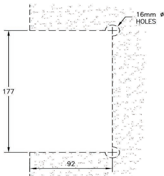
GLASS PREPARATION
