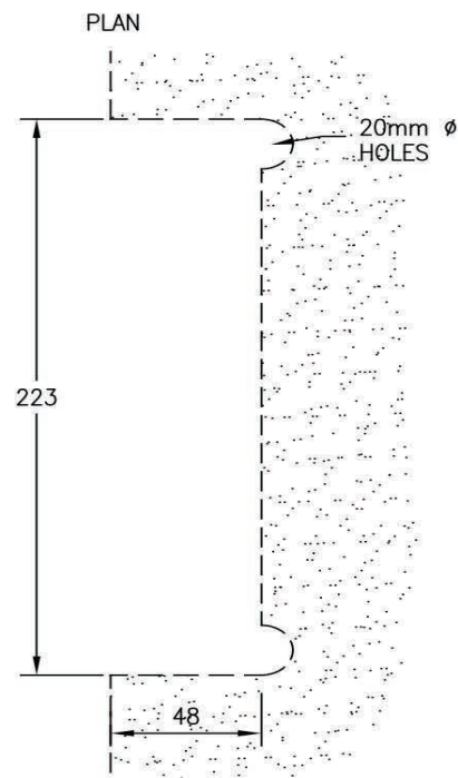
GLASS PREPARATION
