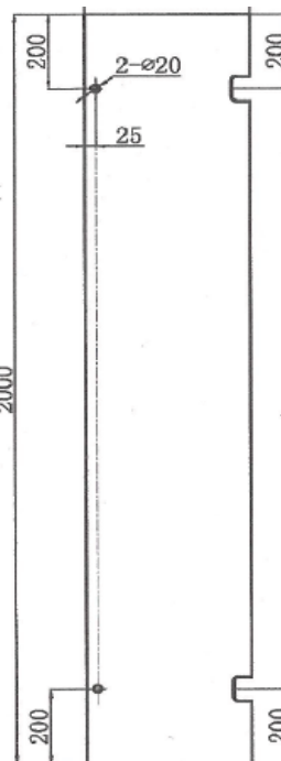
HINGE PANEL
