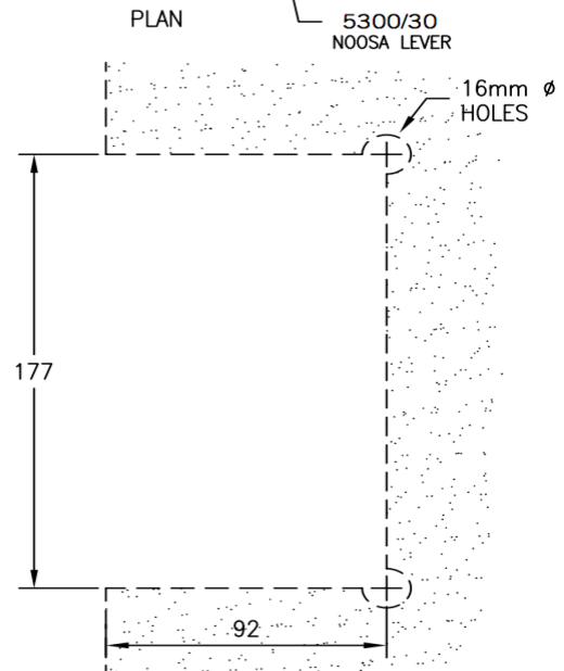
GLASS PREPARATION
