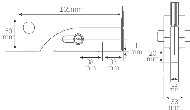
INSITU APPLICATION
