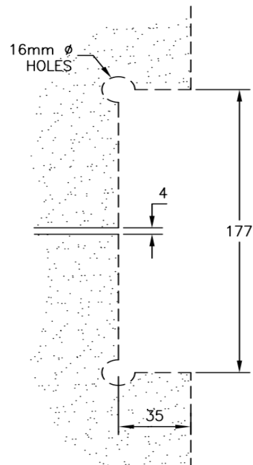
GLASS PREPARATION
