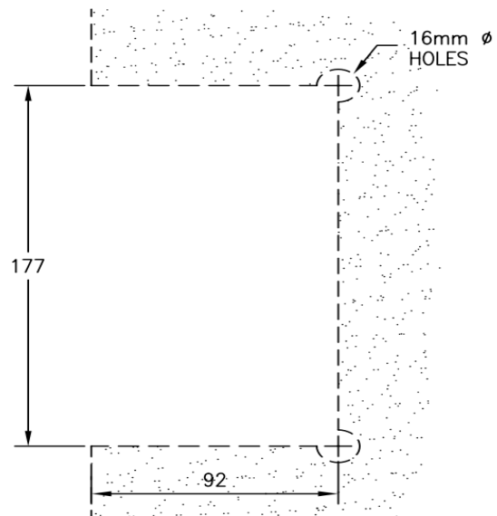
GLASS PREPARATION
