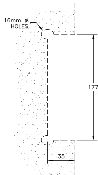
GLASS PREPARATION
