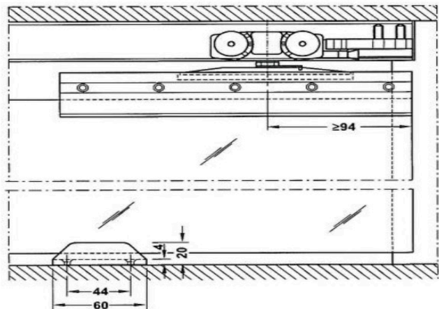
Section guide and trolley hanger
