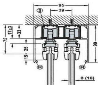
Ceiling installation with double running track and clip panel 90 mm
