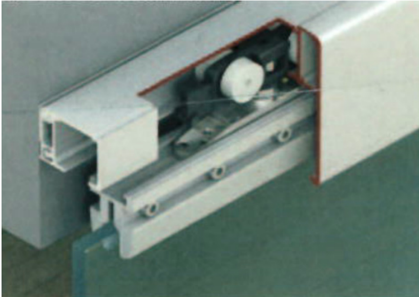
Ceiling installation and wall mounting
