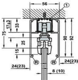
Ceiling installation and wall mounting
