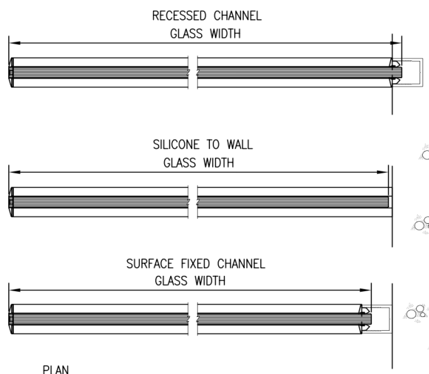
CDS47 BOTTOM
