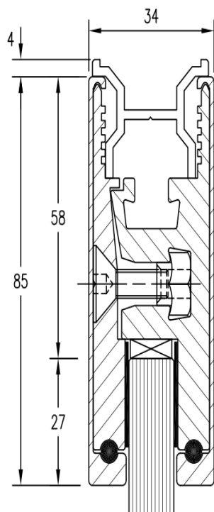
CDS48 TOP
