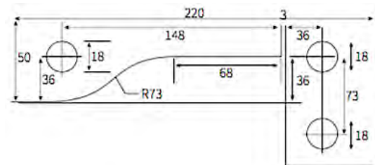
DETAIL / 44400
