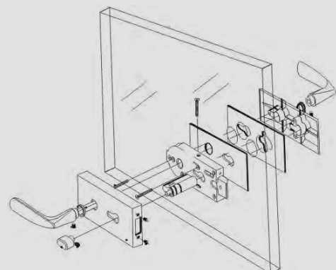
LEVER HANDLE TECHNICAL DIAGRAM
