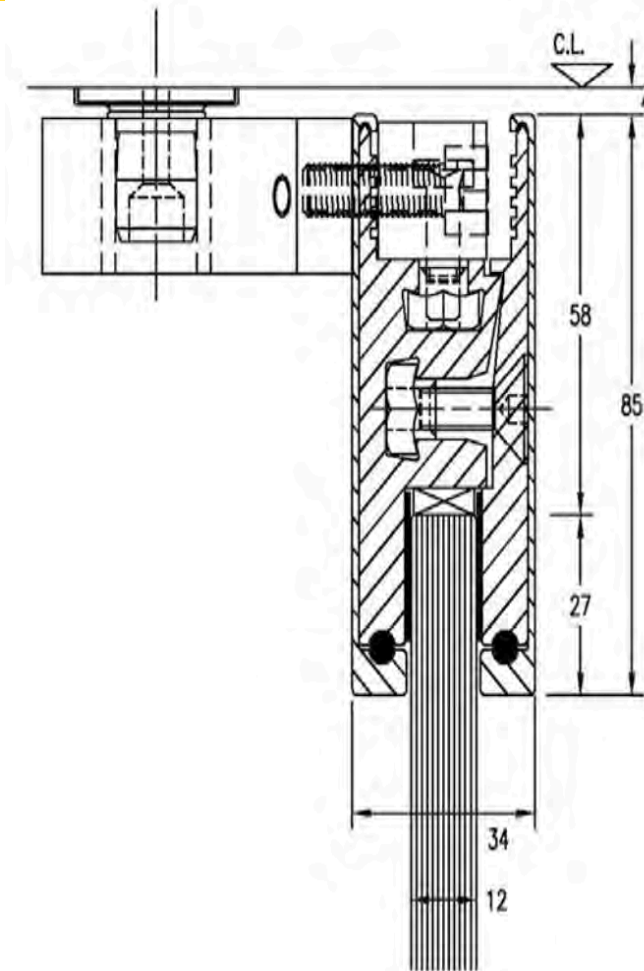
DETAIL
