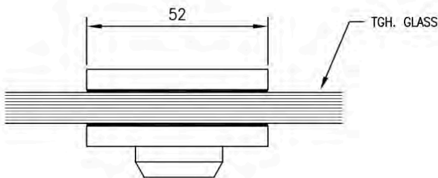
PLAN
