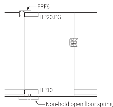
INSITU APPLICATION
