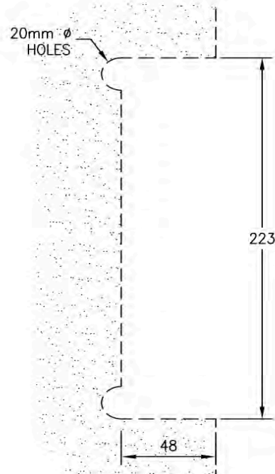
GLASS PREPARATION
