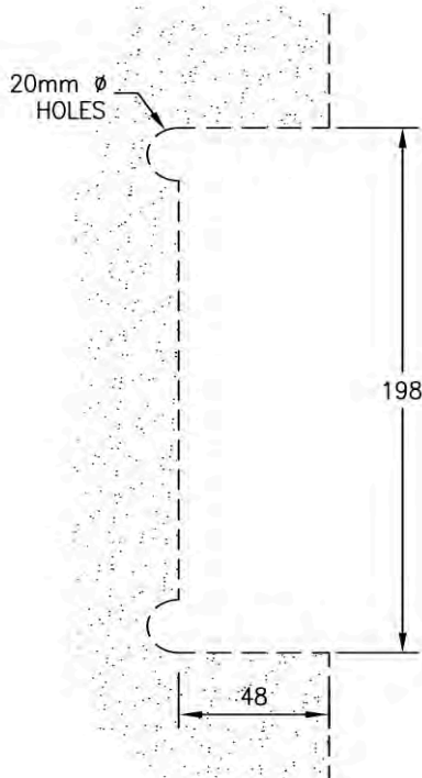
GLASS PREPARATION
