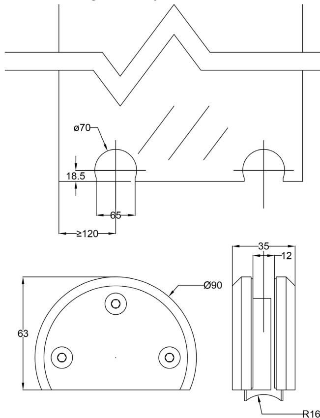
GHA 8300H Bottom Sliding Door System
