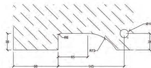
INSITU APPLICATION
