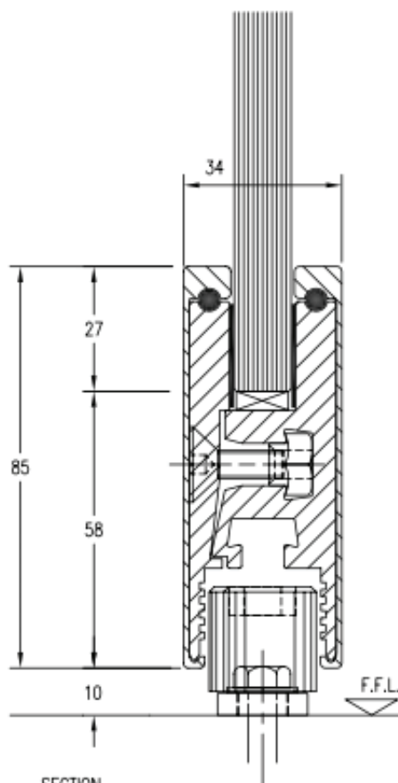
DETAIL
