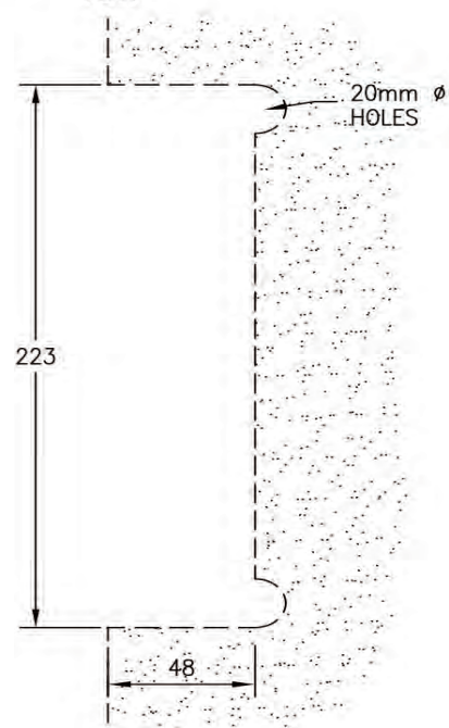
GLASS PREPARATION
