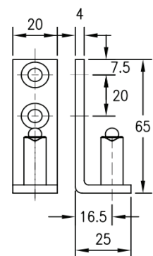
12.009.2 WALL PIVOT
