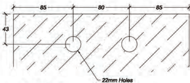
GLASS DETAIL
