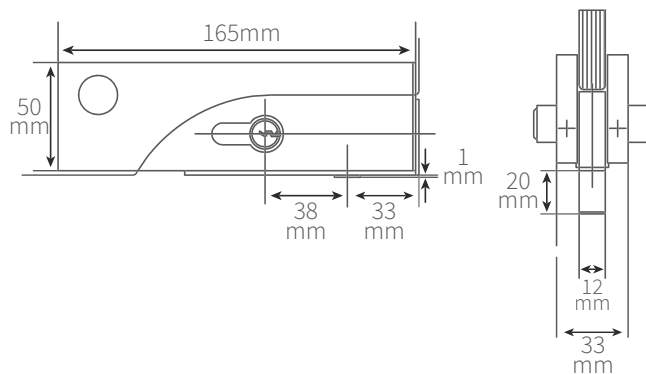
INSITU APPLICATION
