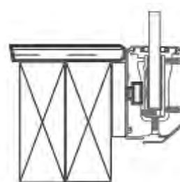
Clamp flush with deck 15mm spacer
