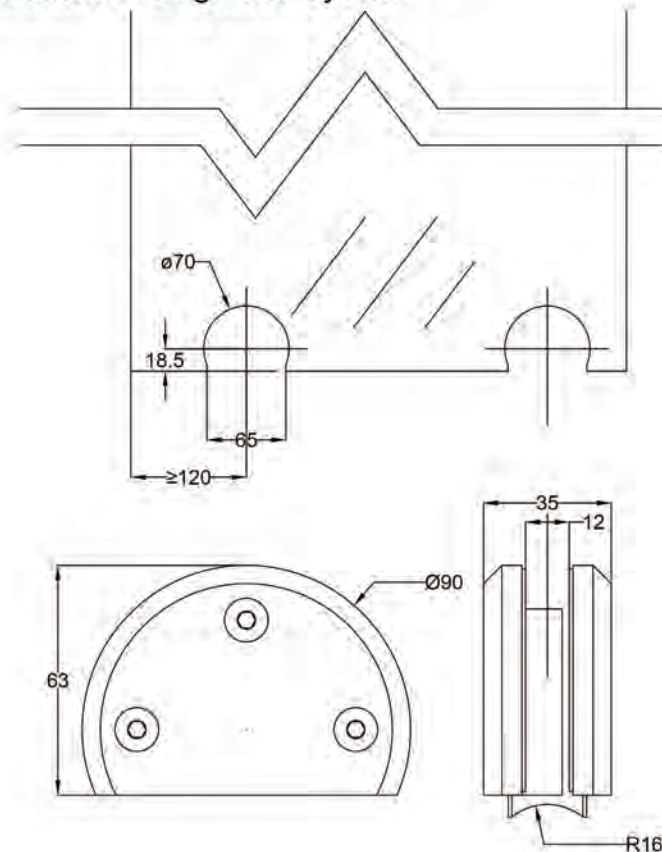
GHA 8300H Bottom Sliding Door System
